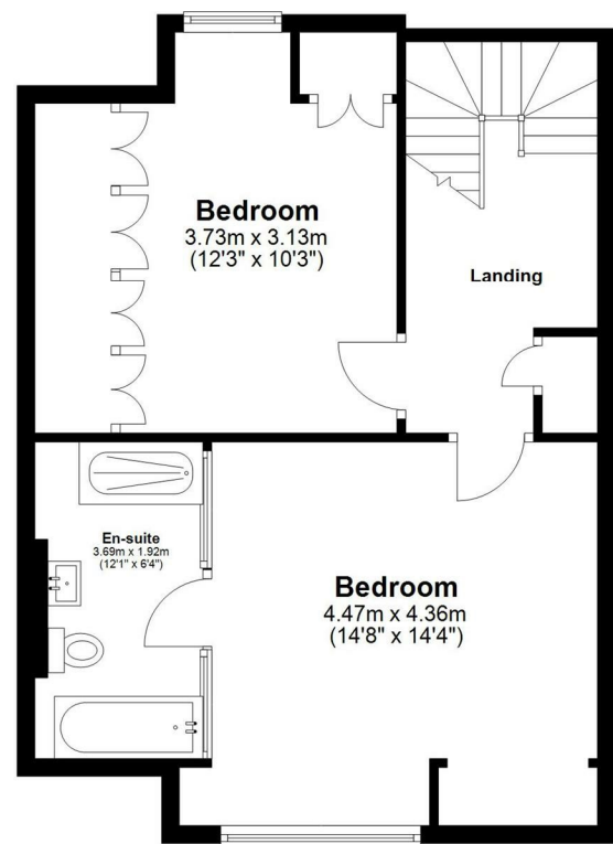
Second Floor Approx. 54.7 sq. metres (588.4 sq. feet)
